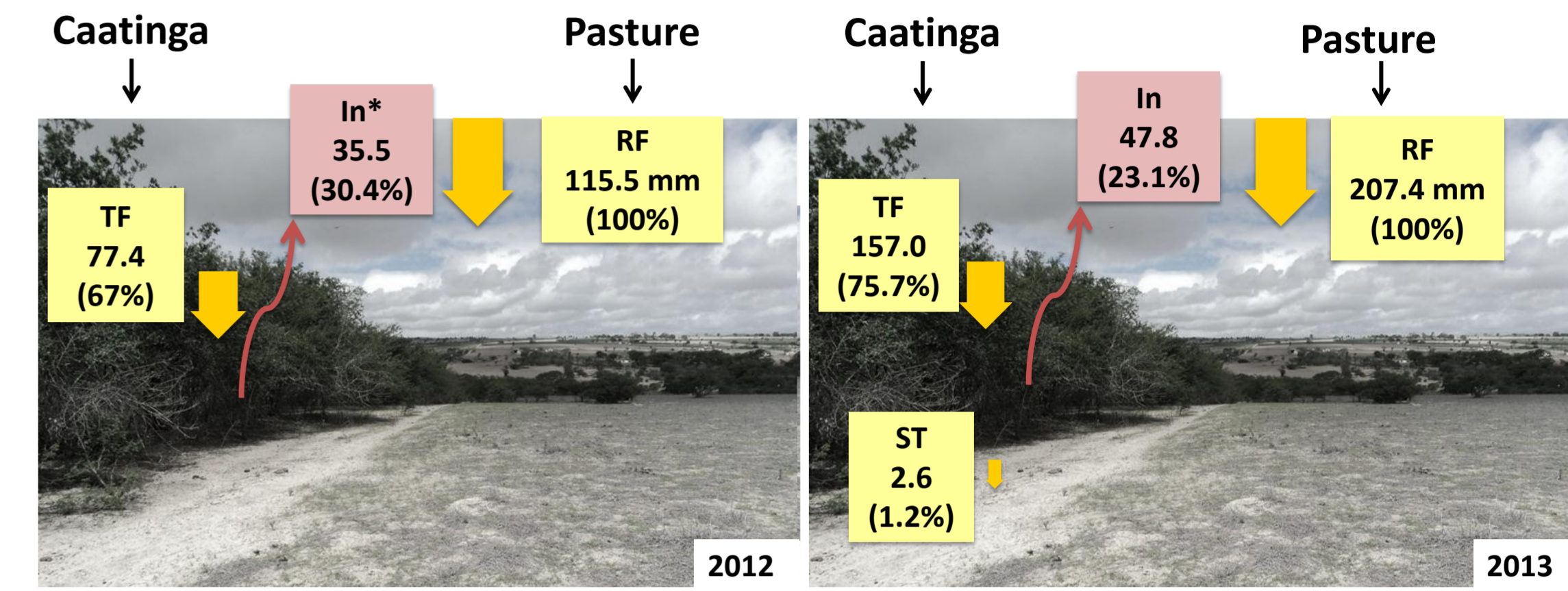
Figure 5: Measured hydrological fluxes in a natural vegetation (Caatinga) and in a pasture. RF: rainfall; In: interception; TF: throughfall; ST: stemflow. Figures are in mm.rainy season -1 and in percentage. *Taking into account the same percentage of stemflow measured in 2013.
